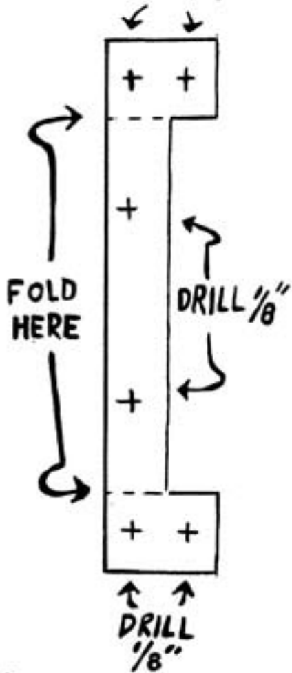
HANG-UP HINGE BRACKET TEMPLATE
