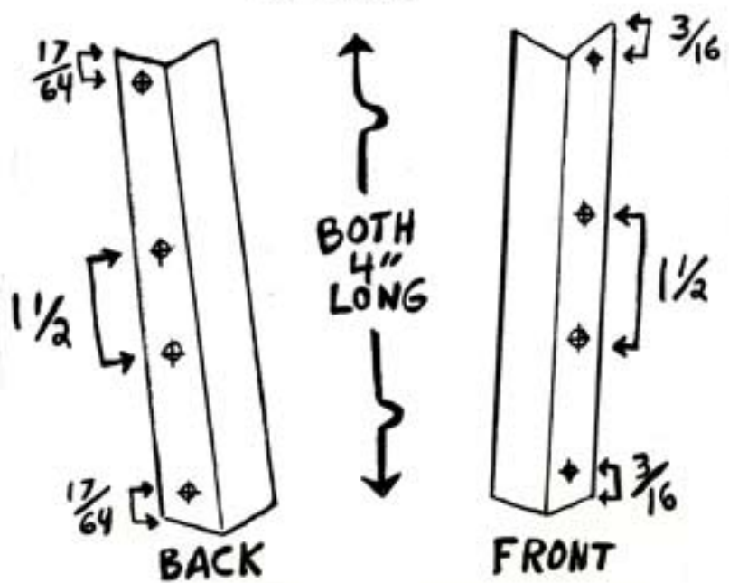
CIRCUIT BOARD BRACKETS
