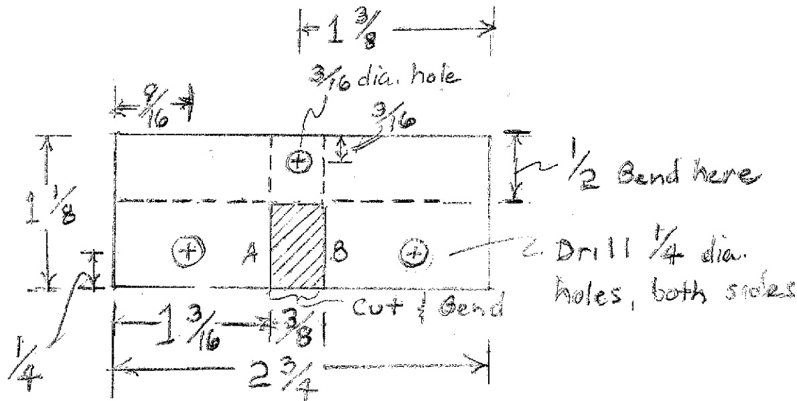
Bracket for Gyrocar (To scale, in inches)
